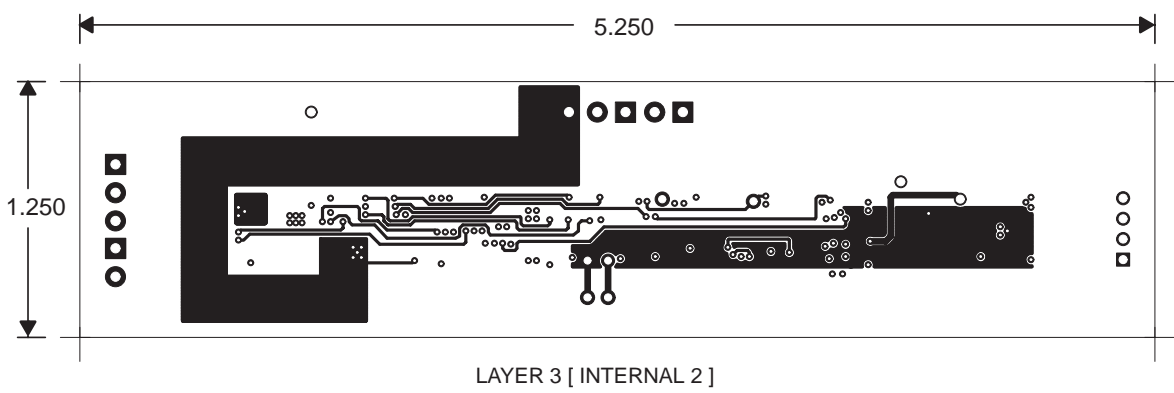
Figure 4-5. Layer 3 (Internal 2)
