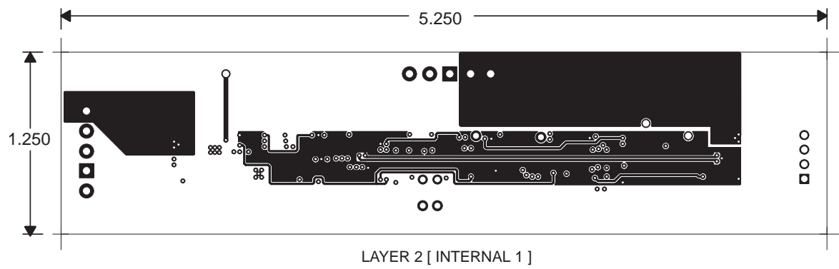
Figure 4-4. Layer 2 (Internal 1)
